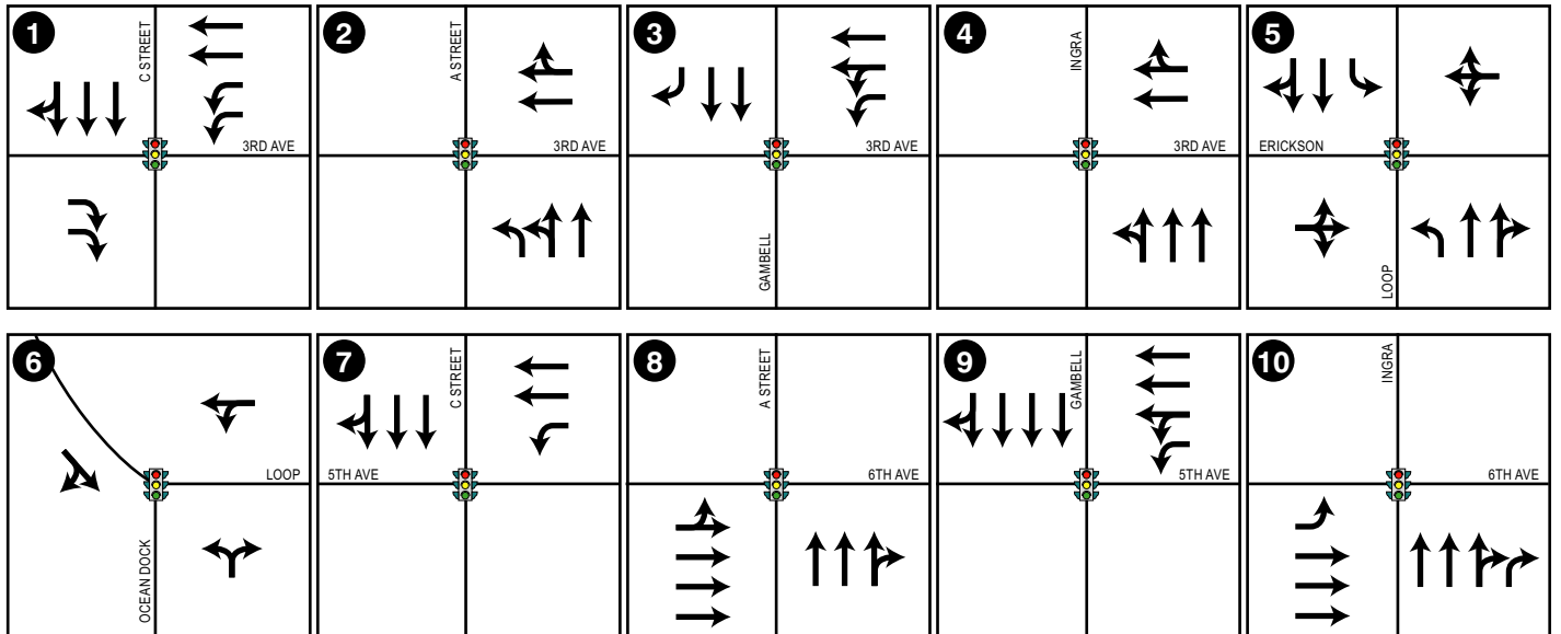
FIGURE 2 ACTION CHANNELIZATION AND TRAFFIC CONTROL KNIK ARM CROSSING
