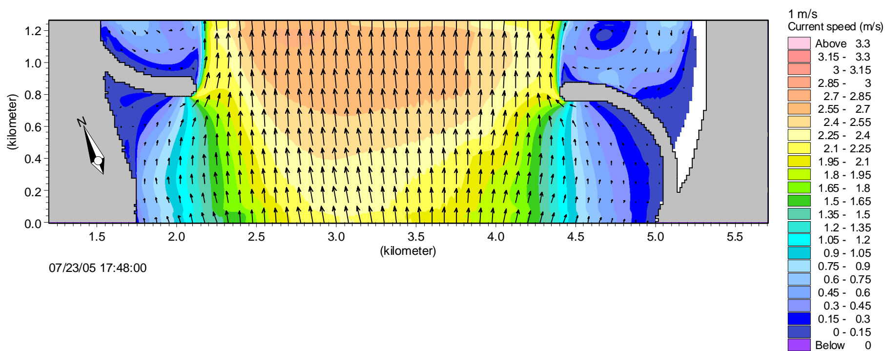
Maximum velocities during flood tide shown occur on 7/23/05 5:48 PM LST = 7/24/05 2:48 AM UTC (LST + 9 hrs)
