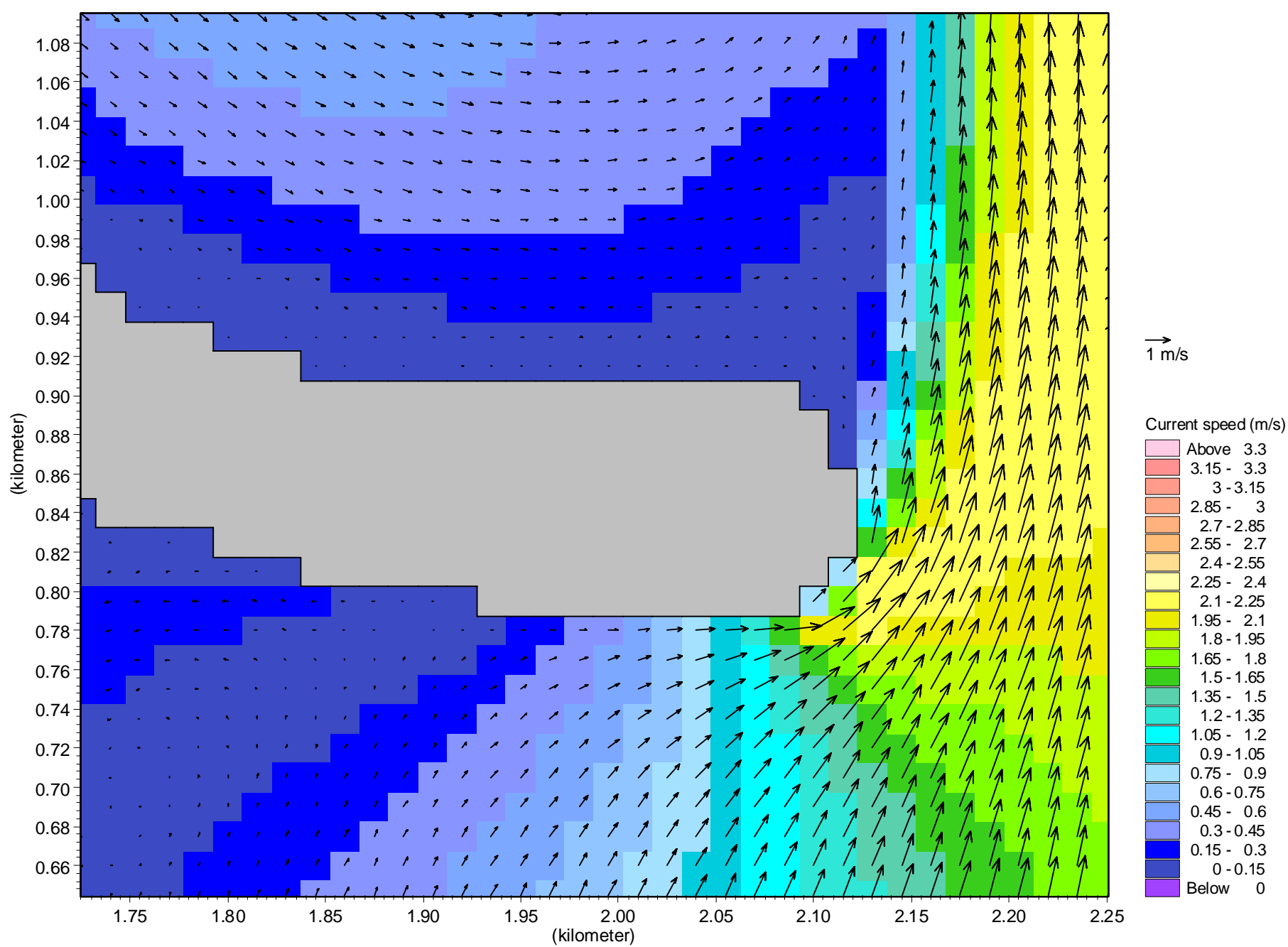
Close-up of western bridge embankment with 15-m grid resolution
