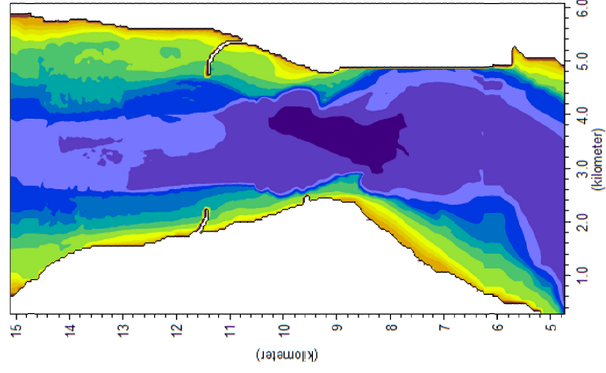
Bathymetry for the Port of Anchorage Expansion and the Proposed 8,200-ft Bridge with Earthen Embankments
