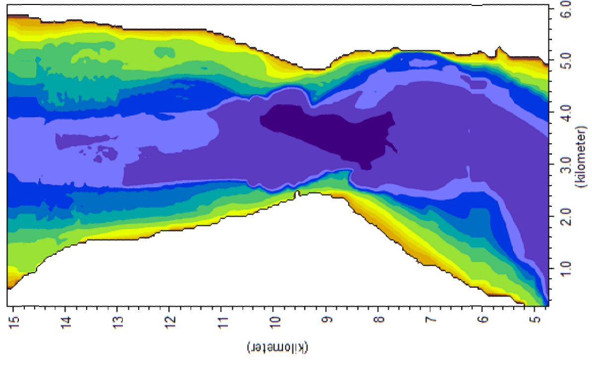
Bathymetry for Existing Conditions (Base Case)
